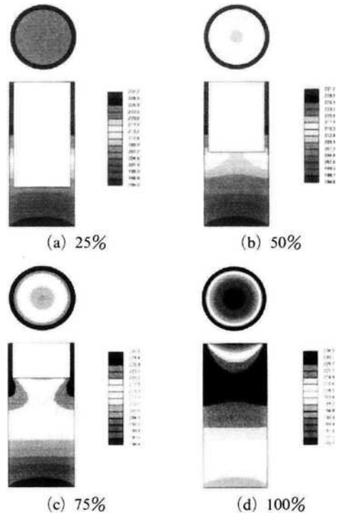
Fig. 8 The temperature distributions with the charge rate
