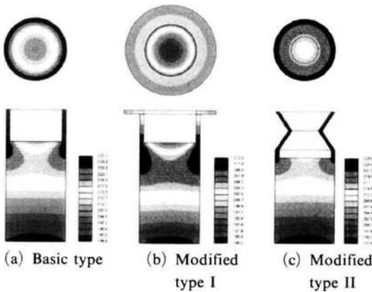
Fig. 14 The temperature distributions with the various crucibles
