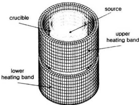
Fig. 2 The configuration of the point-cell source
