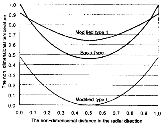
Fig. 15 The temperature variations on the upper face of the source with the various crucibles
